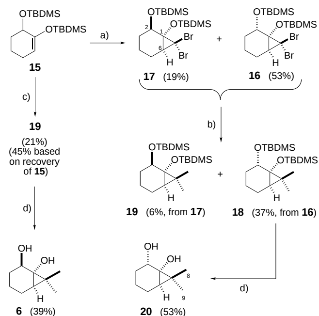
Scheme 4. Synthesis of the epimeric diols 6 and 20 from the enol ether 15 . Reagents and conditions: a) \text{CHBr}_3 (1 equiv, dropwise over 1 h), t\text{BuOK} , pentane, -10^\circ\text{C} →room temperature, 3 h; b) \text{Me}_2\text{CuLi} (4 equiv), \text{Et}_2\text{O} , -23^\circ\text{C} , 3 h, then MeI, -63^\circ\text{C} , 1 h; c) (\text{CH}_3)_2\text{CBr}_2 , n\text{BuLi} , pentane, -78^\circ\text{C} (3 h), -78^\circ\text{C} →room temperature (14 h); d) n\text{Bu}_4\text{NF} , THF, reflux, 2 h.
